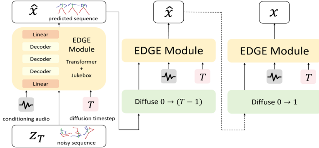
Figure 3: Music2motion
