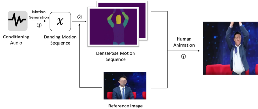
Figure 2: Music2motion
