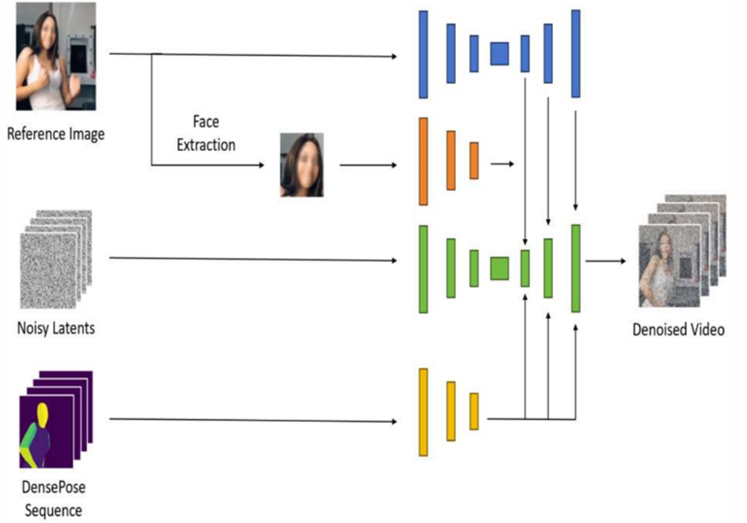
Figure 6: Our Model Architecture.
