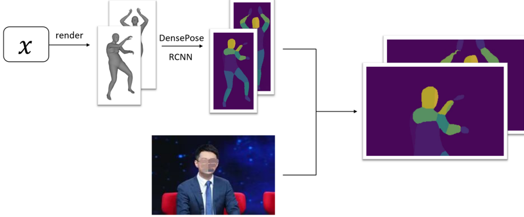
Figure 4: Motion Alignment Pipeline.
