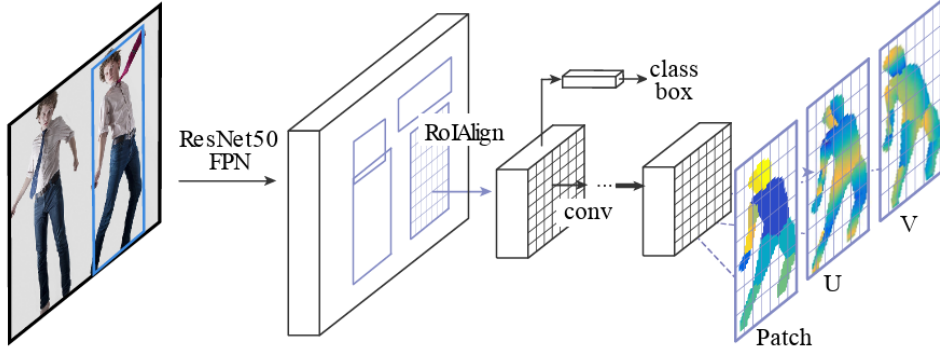
Figure 5: Densepose R-CNN.[6]
